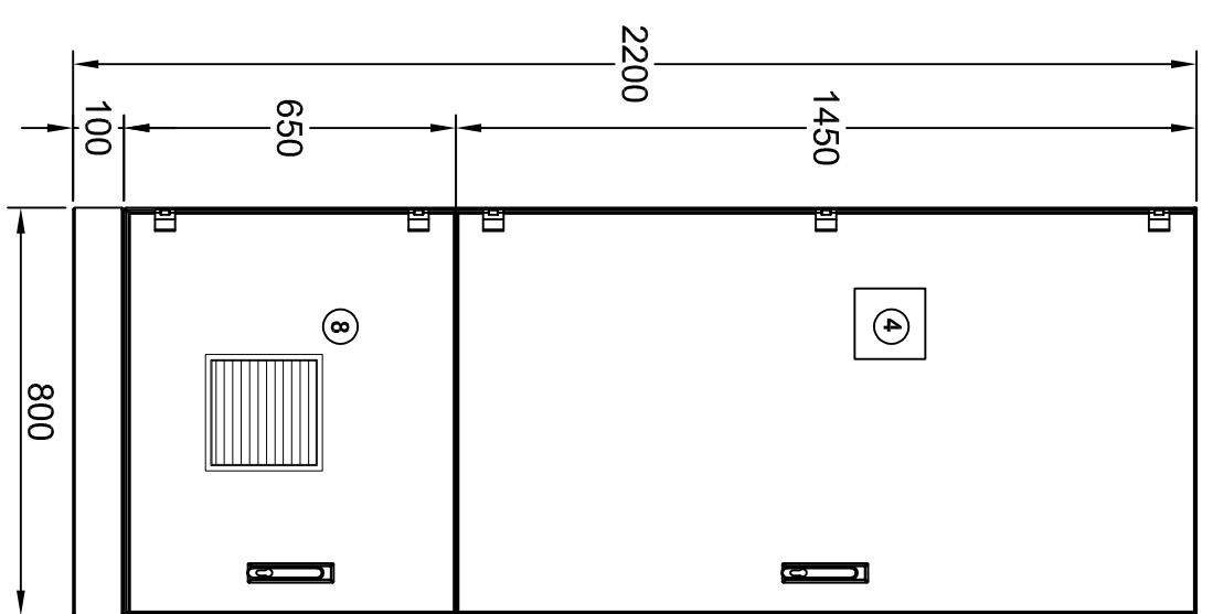
Vista Frontal Exterior
